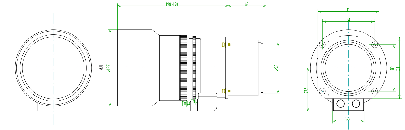
Standard Zoom Lens (Mid Zoom) F=97-131mm F1.7-2.7 Lens Shift 1:8
