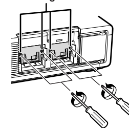
Securing screws
